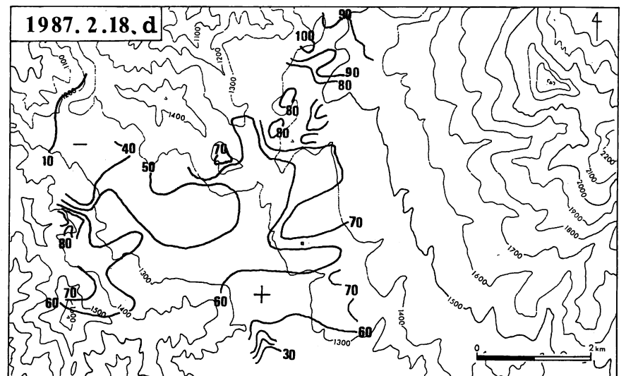
Fig. 5. Distribution of snow depth (cm) at Sugadaira for (a) Feb. 25, 1983, (b) Feb. 25, 1984, (c) Feb. 2, 1986 and (d) Feb. 18, 1987.
