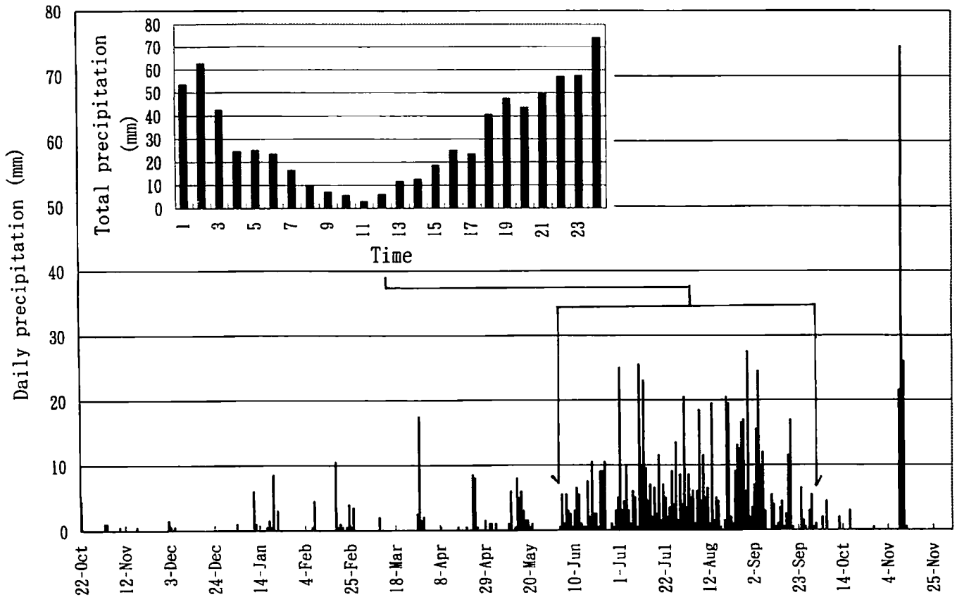
Fig. 3 Daily precipitation change in 1994–95. Upper figure shows diurnal variation of hourly precipitation accumulated from June 3 to October 1, 1995.
