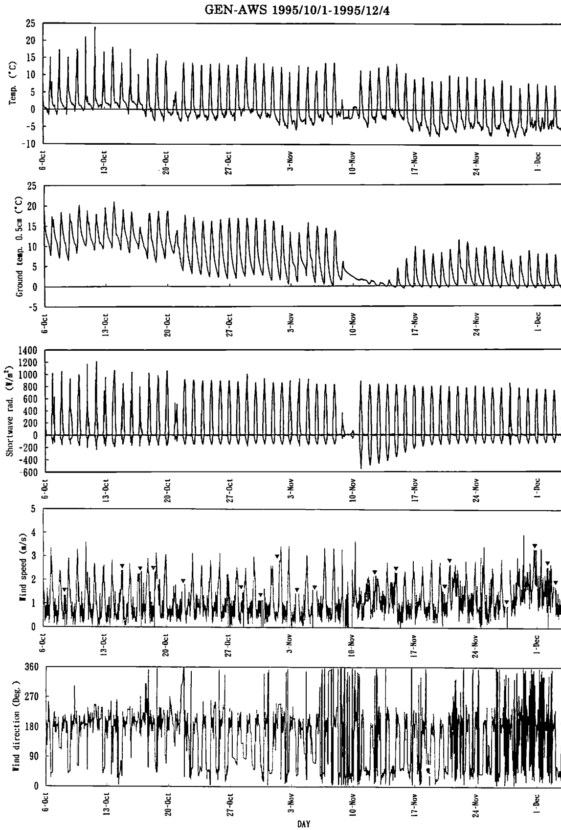
Fig. 5 Same as Fig. 4, but from October 6 to December 3, 1995.
