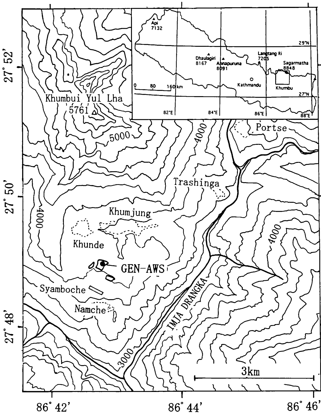
Fig. 1 Location of the GEN-AWS in Khumbu area.
