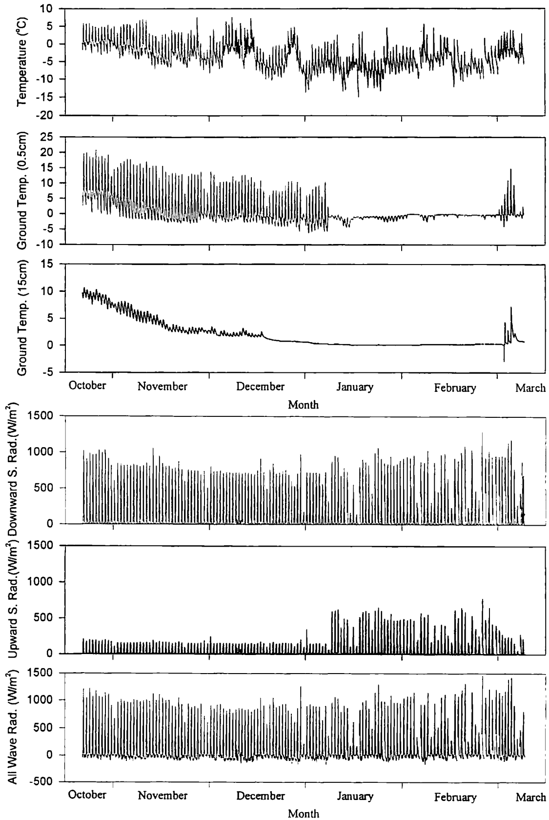
Fig. 4 Time sequences of meteorological elements observed with Aanderaa-AWS with 30 minutes interval, from Oct. 22, 1994 to March 3, 1995.
