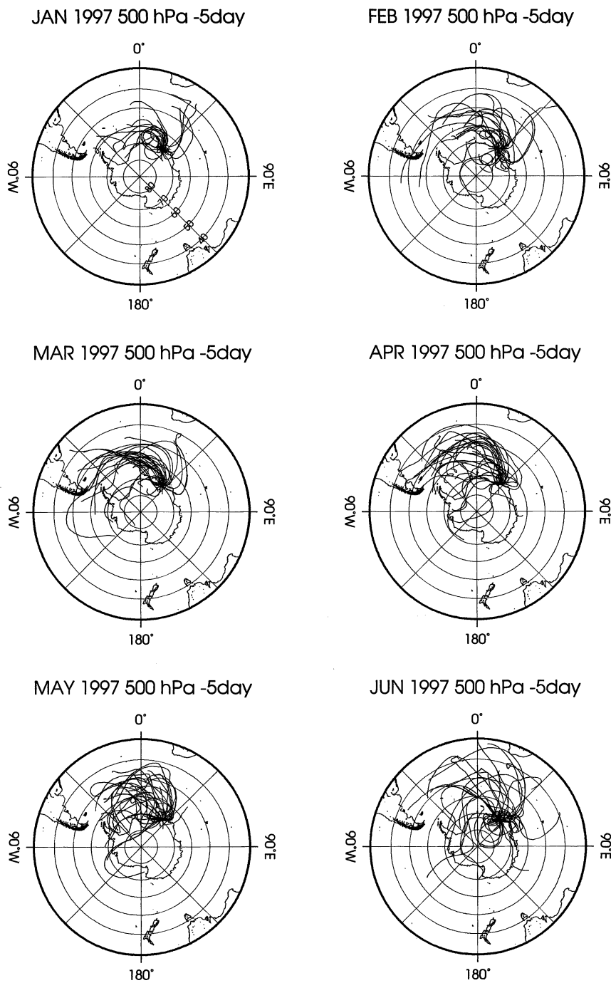
Fig. 1a. Horizontal distribution of backward trajectories that reached a height of 500 hPa over Syowa Station in 1997. Calculations ended either at 5 days or when a trajectory crossed a mountain or sea surface.
