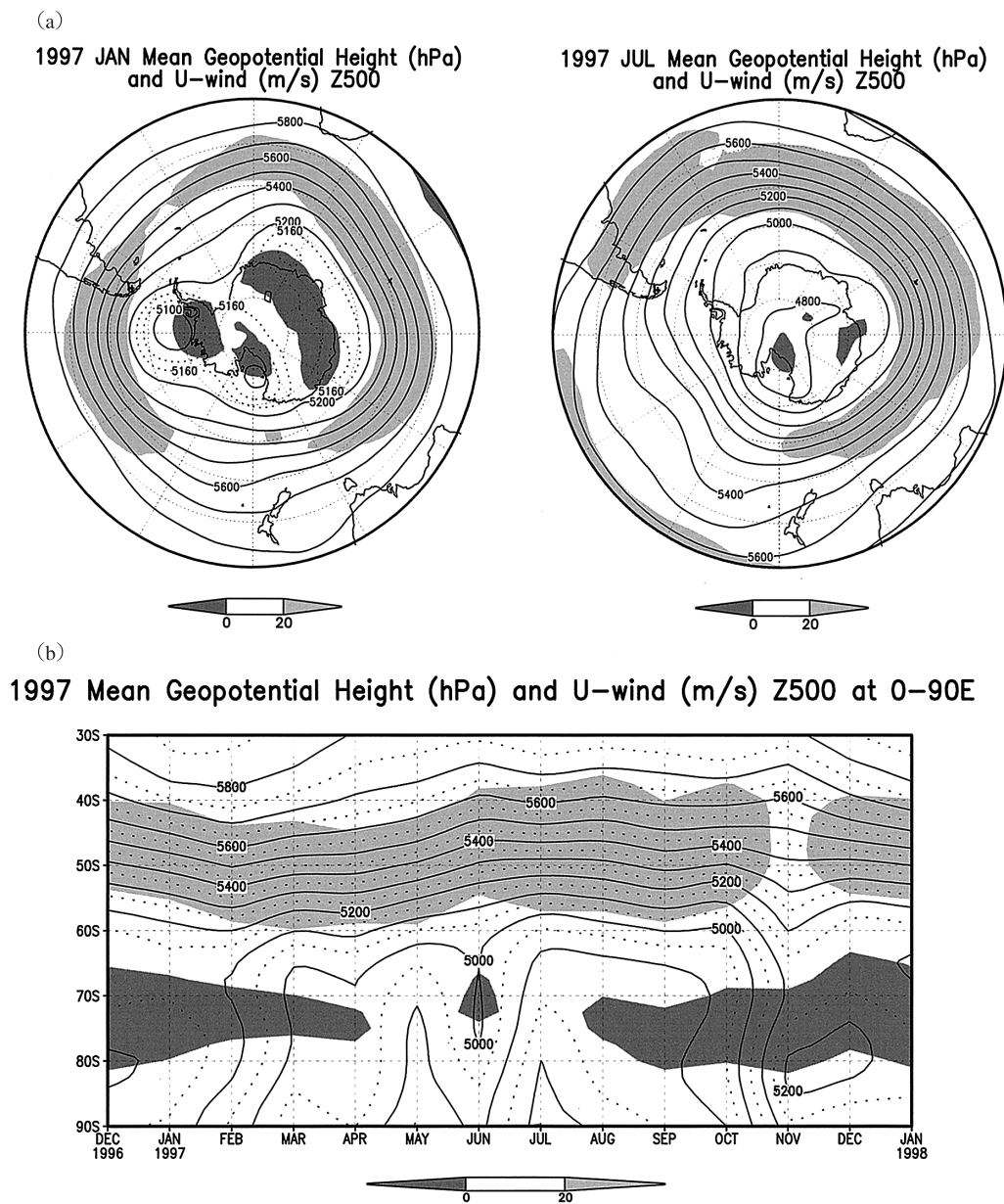
Fig. 3. (a) Monthly averaged geopotential height (contoured) and zonal wind (shaded) at the 500 hPa level (referred to as Z500) in January and July. The contour interval for the solid lines is 100 m. The lines for 5130 and 5160 m are dotted. Dark shading is easterly wind and light shading is westerly wind.
