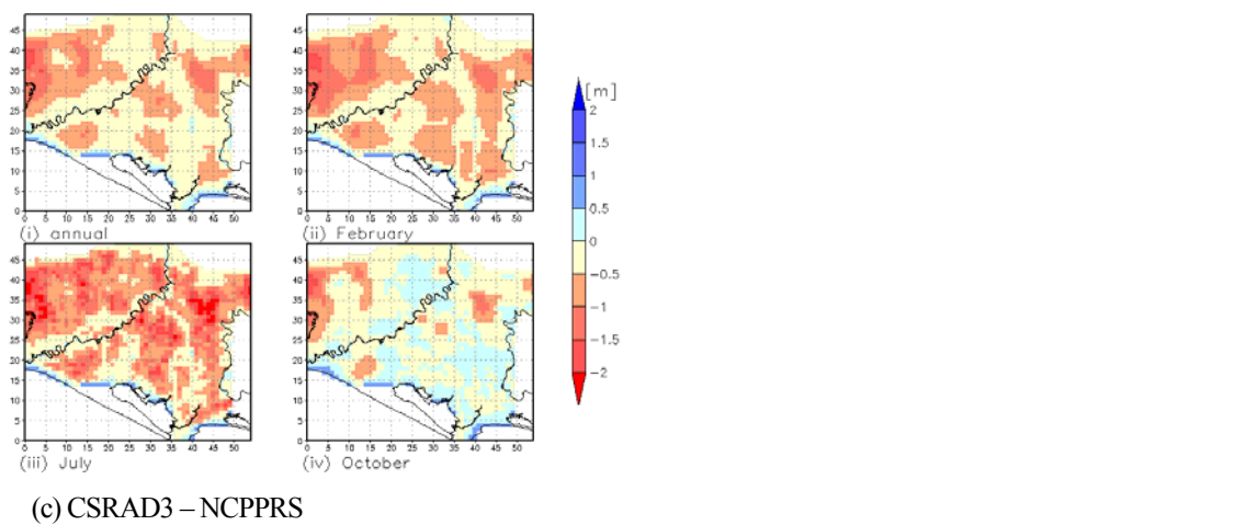
Fig. 10. Differential of groundwater level (annual mean and monthly mean of February, July and October)
