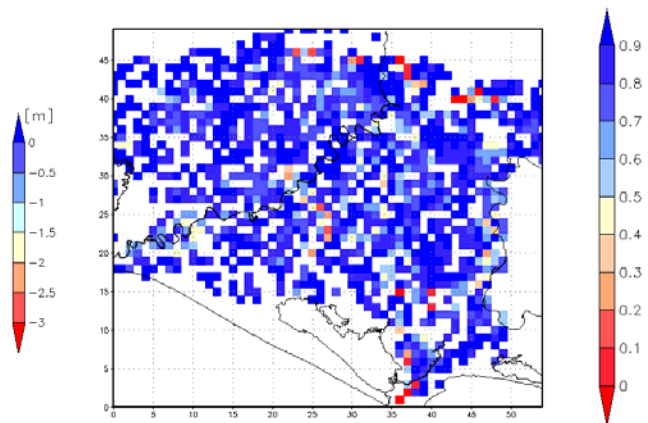
Fig. 7. Annual Ta/Tp in NCPPRS (10-year mean)
