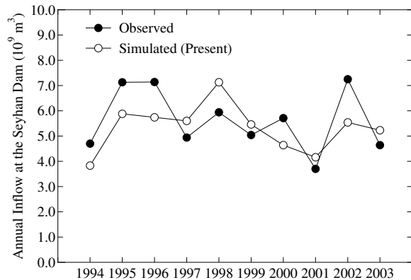
Fig.3 Annual inflow at the Seyhan Dam.
