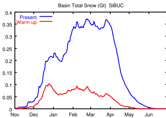
Fig.10 Basin total storage of snow.
