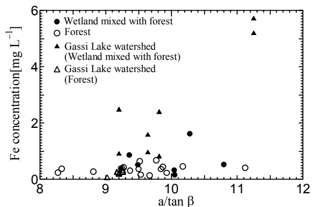
Figure 4. Fe concentration plotted against mean a/tanβ of each catchment
