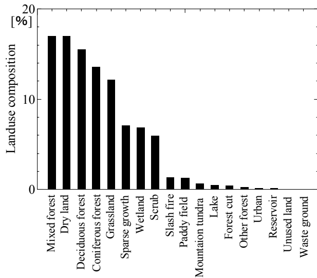
Figure 2. Landuse composition of the Amur river basin
