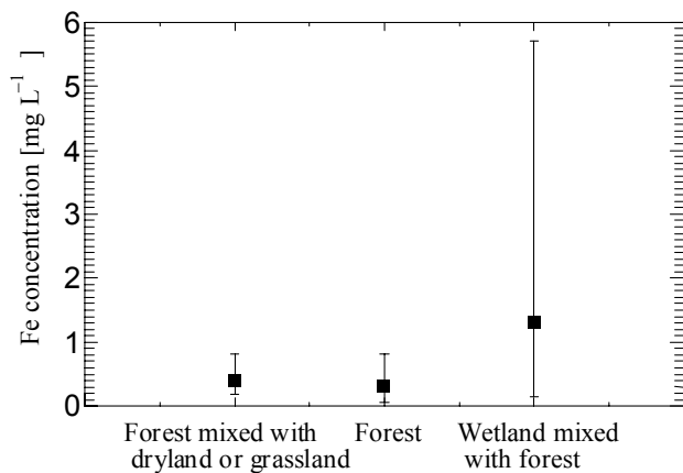
Figure 3. Fe concentration range plotted against landuse pattern of catchment area
