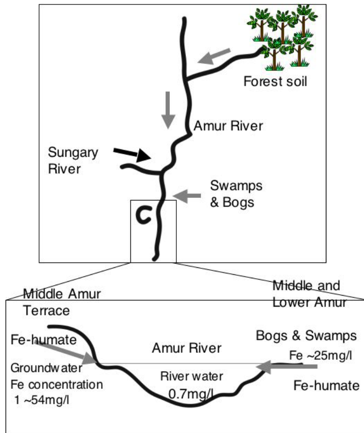
Fig.1 Schematic illustration of sources of iron in the Amur River system. The iron concentration was taken from Schesterkin (2004)
